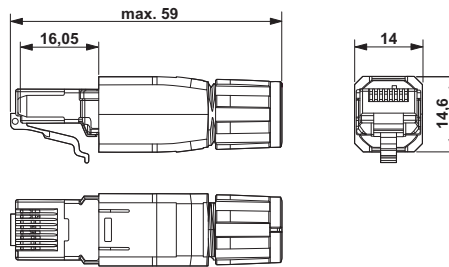
RJ45 connector, IP20
