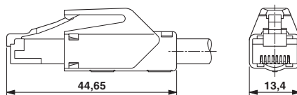
Dimensioned drawing
