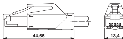
Dimensioned drawing
