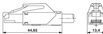
RJ45 connector, IP20
