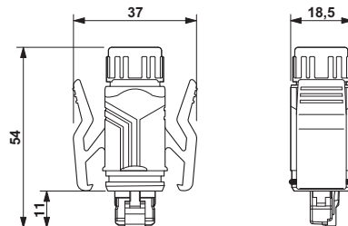
RJ45-connector, IP67
