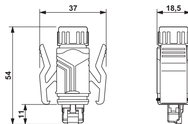
RJ45-connector, IP67
