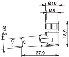
Dimensioned drawing
