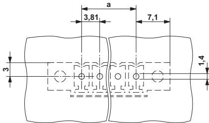
Drilling diagram
