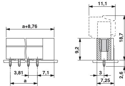
Dimensioned drawing
