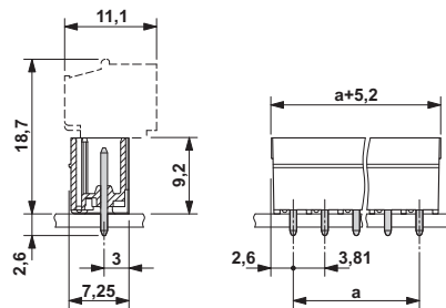
Dimensioned drawing
