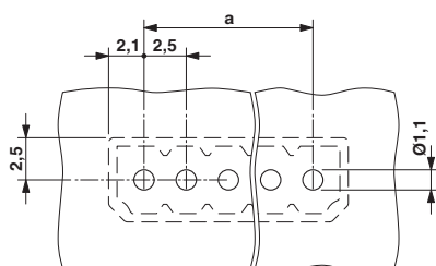
Drilling diagram
