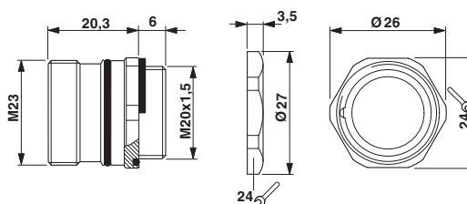
Dimensioned drawing
