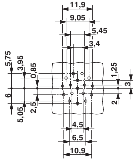
Drilling diagram
