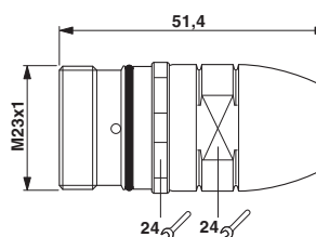
Dimensioned drawing
