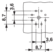
Drilling diagram
