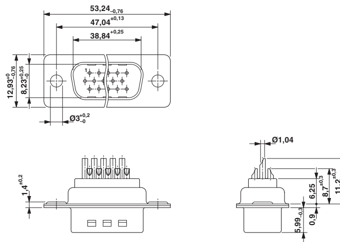
Dimensioned drawing
