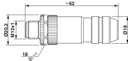
Plug, M12 x 1, straight, shielded
