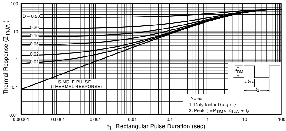
Fig 20. Maximum Effective Transient Thermal Impedance, Junction-to-Ambient
