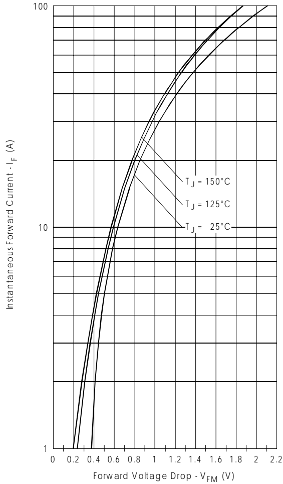
Fig. 17 - Maximum Forward Voltage Drop Characteristics
