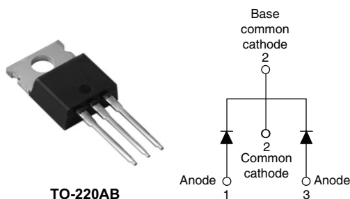
TO-220AB
