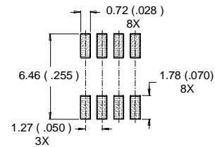
RECOMMENDED FOOTPRINT
