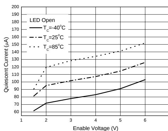
Figure 5. Quiescent Current vs. Enable Voltage
