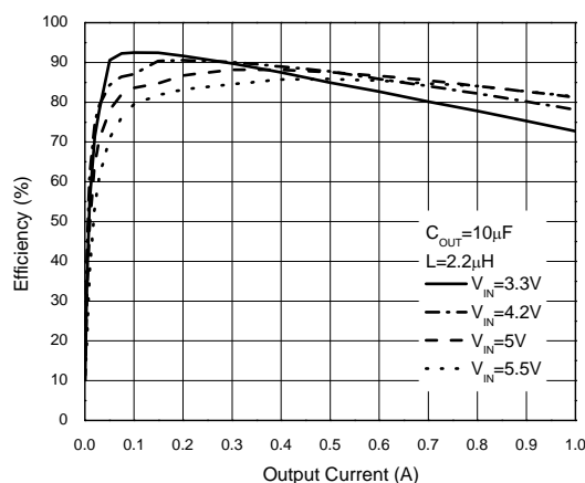
Figure 5. Efficiency vs. Output Current ( V_{OUT}=2.5V )
