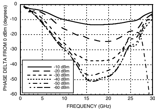
Phase Linearity over Frequency @ 85 C Temperature [1]
