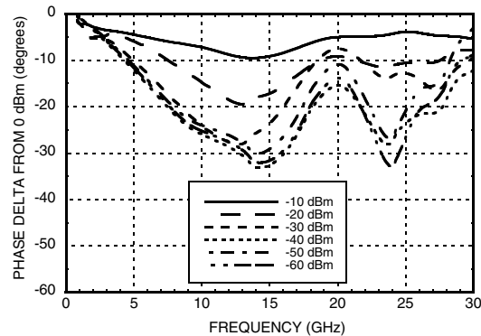
Phase Linearity over Frequency @ -40 C Temperature [1]
