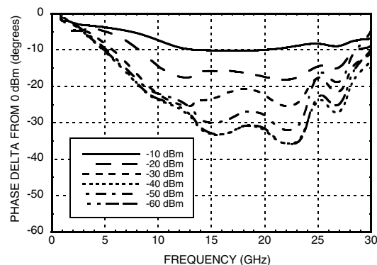
Phase Linearity over Frequency @ 25 C Temperature [1]
