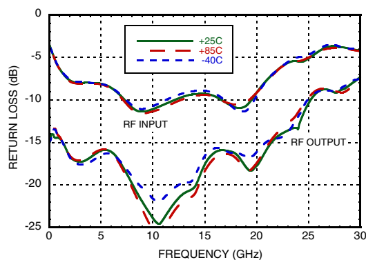
Return Loss vs. Frequency Over Temperature [1]
