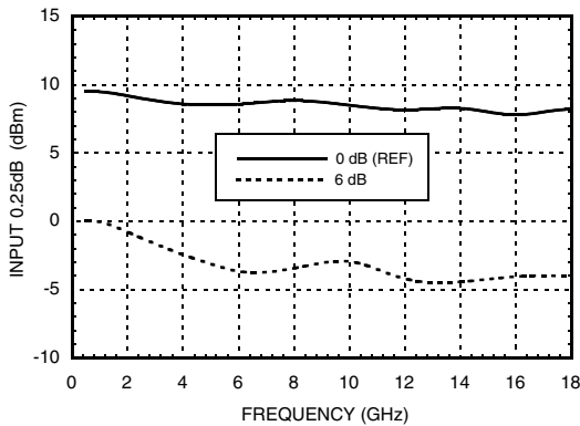
0.25 dB Compression vs. Attenuation
