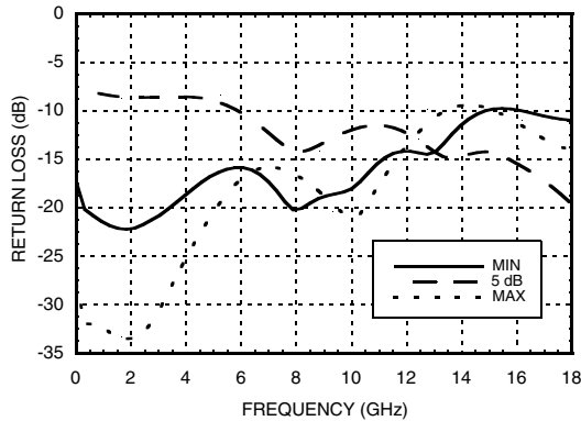
Return Loss vs. Attenuation
