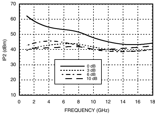
Input IP2 vs. Attenuation*
