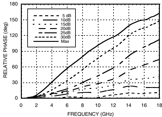
Relative Phase vs. Attenuation
