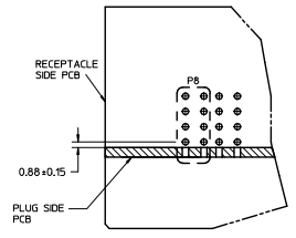
PARTIAL SECTION Z-Z SCALE 3:1
