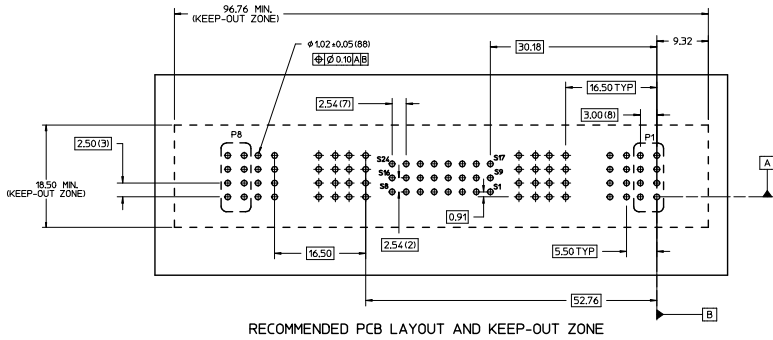
RECOMMENDED PCB LAYOUT AND KEEP-OUT ZONE
