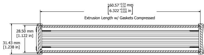
SECTION Y-Y
