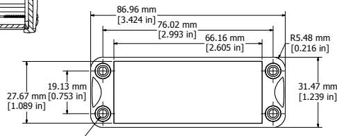
END PANEL - VIEW FROM OUTSIDE
