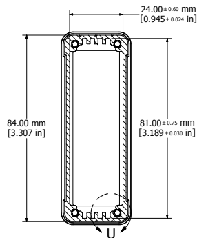
SECTION T-T
