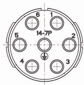
Size 14-7 6 + Grounding
