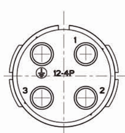
Size 12-4 3 + Grounding
