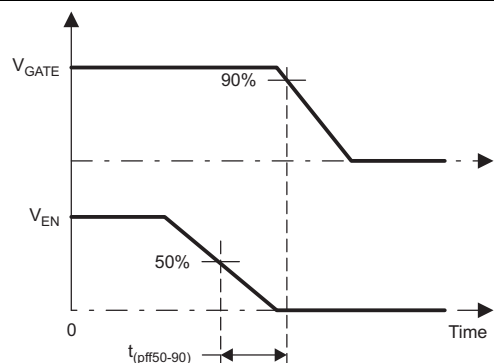
Figure 28. t_{pff50-90} Timing Definition
