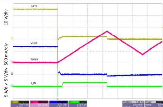
Figure 35. Current Limit During Output-Load Short-Circuit Condition (Overview)
