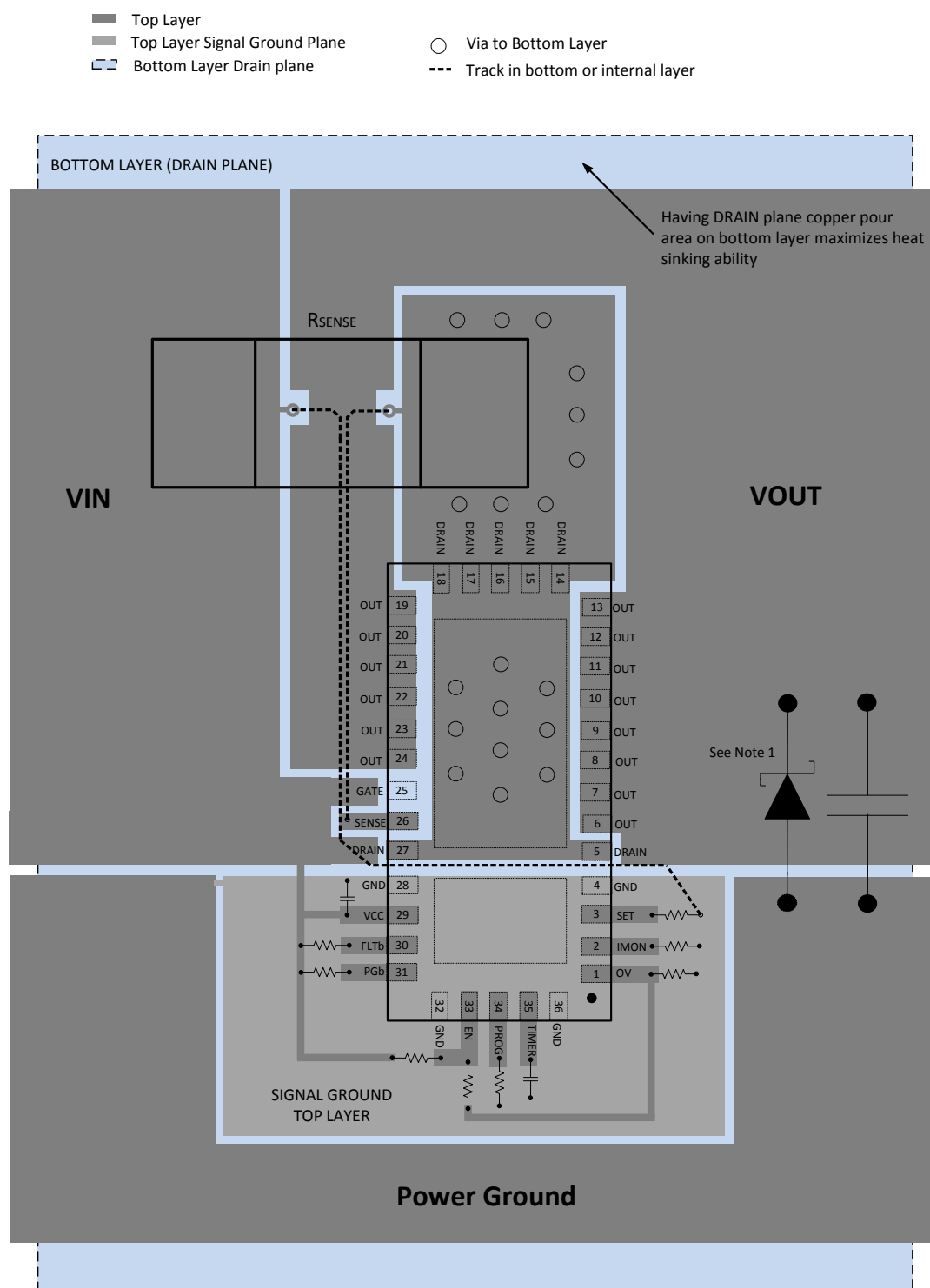
Figure 51. Layout Example
