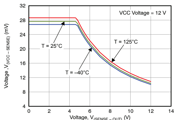
Figure 4. Voltage Across R_{SENSE} in Inrush Power Limiting vs V_{DS} of internal FET
