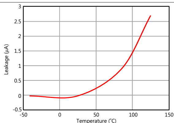
Figure 26. Leakage Current vs Temperature
