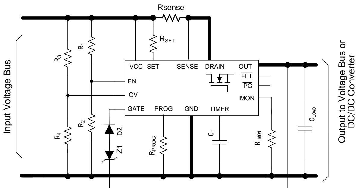
Figure 47. Negative Voltage Gate Protection
