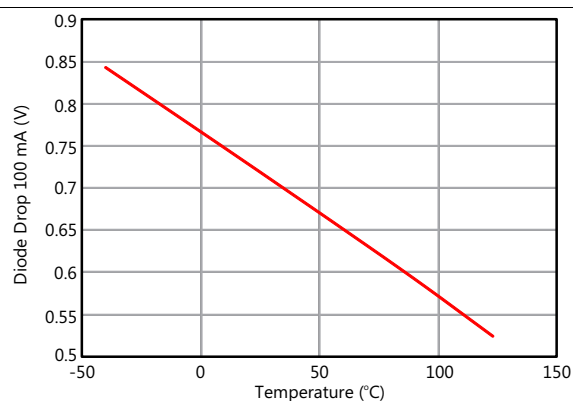
Figure 24. Diode Drop vs Temperature
