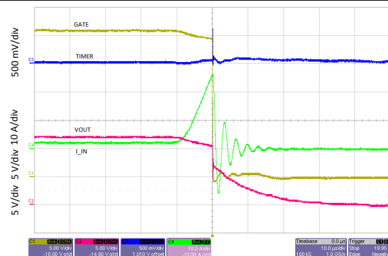
Figure 36. Current Limit During Output-Load Short-Circuit Condition (Onset)
