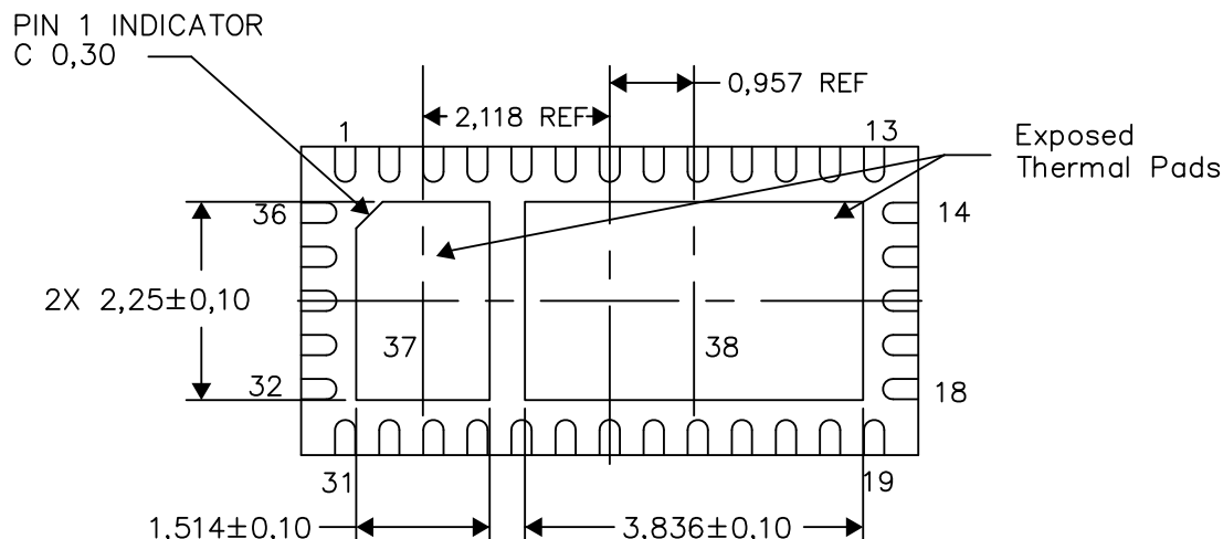
Bottom View
