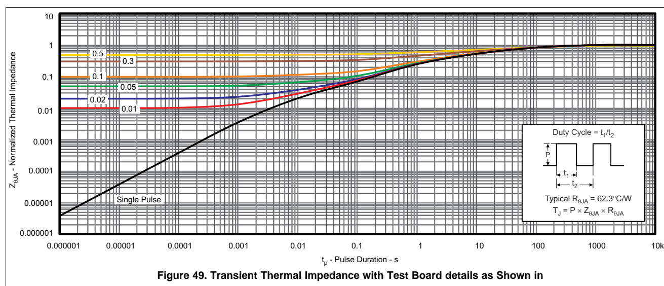
Board Details - Thermal Impedance Characteristic
