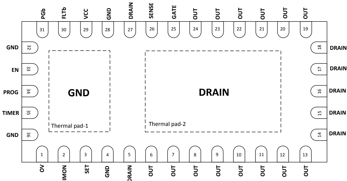
Pin Functions
