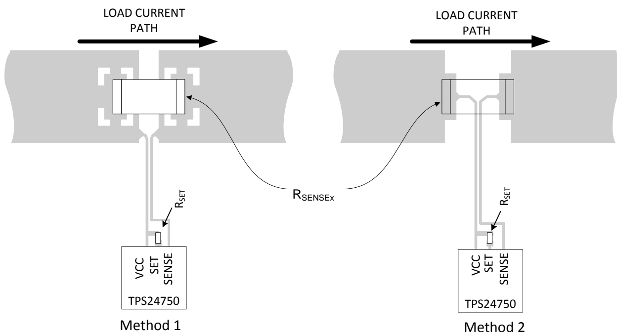
Figure 50. Recommended R_{SENSE} Layout
