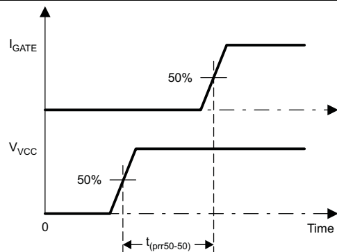
Figure 29. t_{pr50-50} Timing Definition
