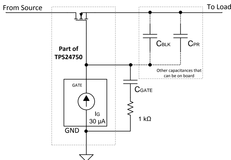
Figure 43. Gate Capacitor (dV/dt) Control Inrush Mode.
