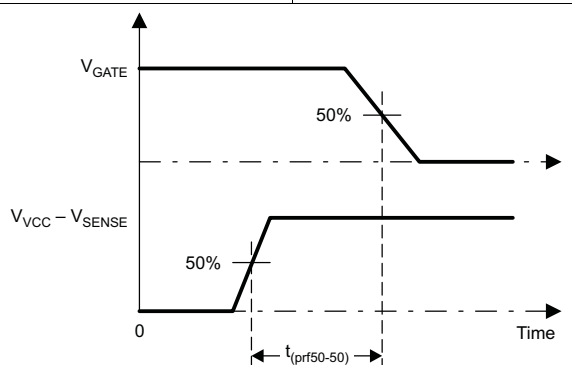
Figure 30. t_{prf50-50} Timing Definition
