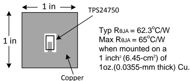
Board Details - Thermal Impedance Characteristic
