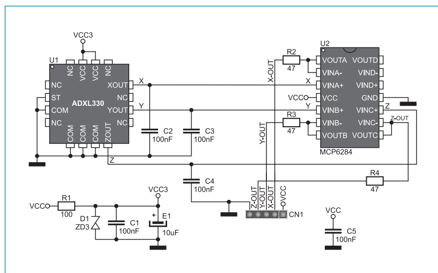
Figure 3: Accel Board connection schematic
