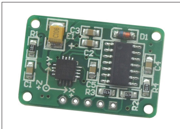
Figure 1: Accel Board
