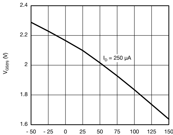
Threshold Voltage
