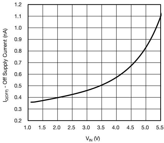
Figure 6 - Off Supply Current vs. Input Voltage
