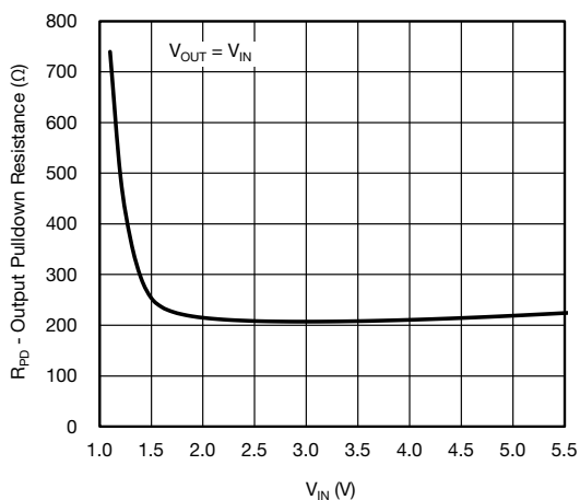
Figure 12 - Output Pulldown Resistance vs. Input Voltage
