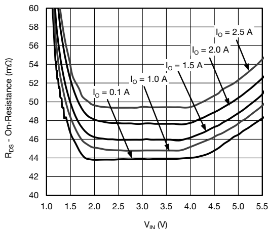
Figure 11 - On-Resistance vs. Input Voltage
