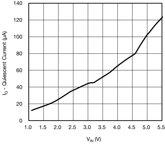
Figure 5 - Quiescent Current vs. Input Voltage
