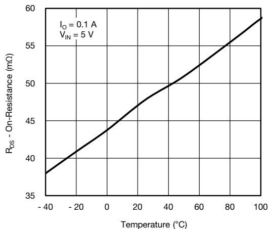
Figure 13 - On-Resistance vs. Temperature
