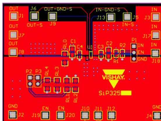
Figure 32 - Evaluation Board Layout for TSOT23-6L
