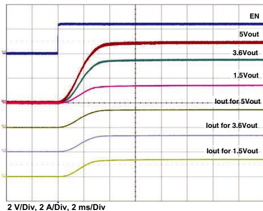
Figure 22 - Typical Turn-on Delay, Rise Time C_{OUT} = 200 \mu F, C_{IN} = 4.7 \mu F, I_{OUT} = 1.5 A
