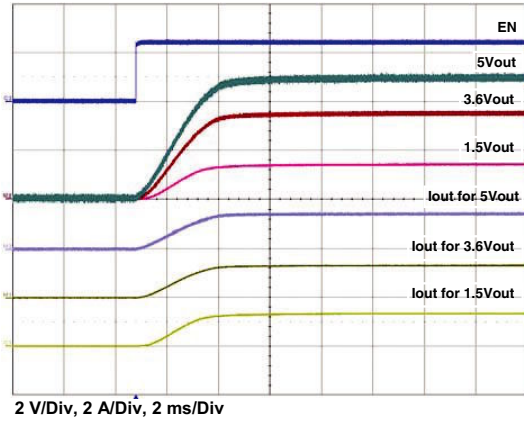
Figure 20 - Typical Turn-on Delay, Rise Time C_{OUT} = 0.1 \mu F, C_{IN} = 4.7 \mu F, I_{OUT} = 1.5 A
