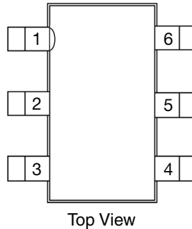
Figure 3 - TSOT23-6 Package
