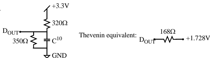
Figure B: 3.3V Output load
