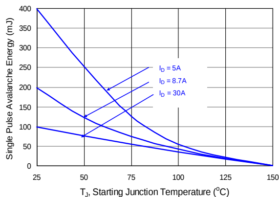
Figure 22: Q1 & Q3 Single Pulse Avalanche Energy
