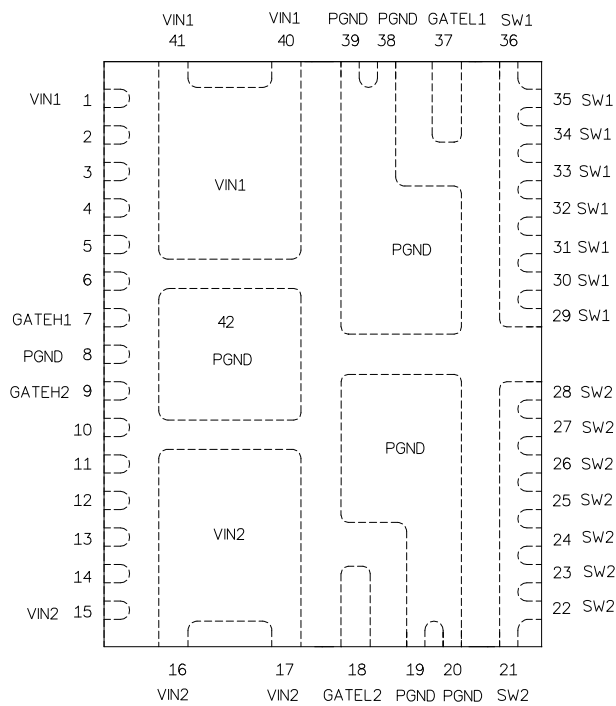
Figure 1: IRF3546 Top View
