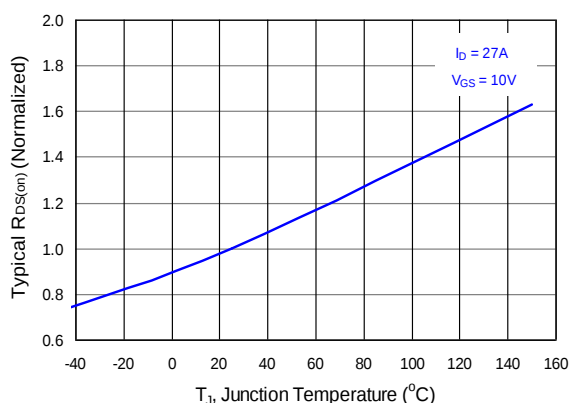
Figure 11: Q1 & Q3 On-Resistance vs. Temperature
