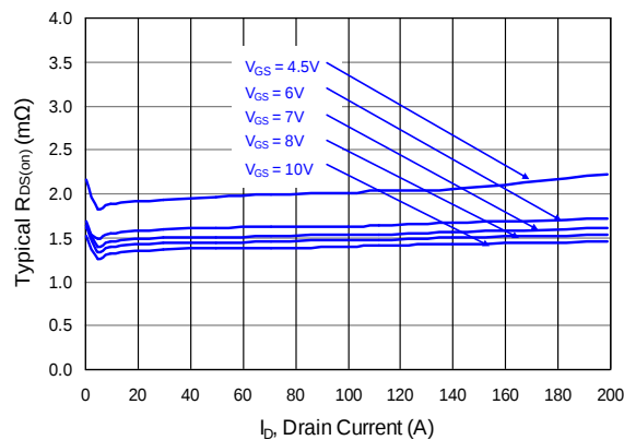
Figure 19: Q2 & Q4 Typical On-Resistance
