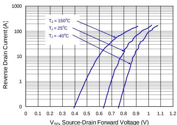
Figure 17: Q1 & Q3 Drain-Source Diode Characteristics
