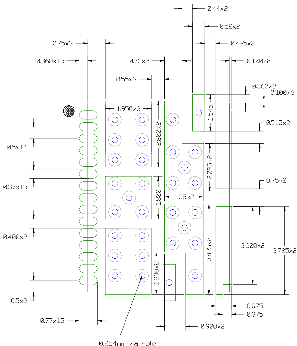
Figure 29: Solder Resist
