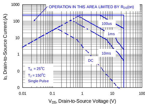
Figure 24: Q1 & Q3 Maximum Safe Operating Area
