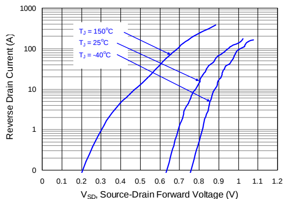
Figure 20: Q2 & Q4 Drain-Source Diode Characteristics
