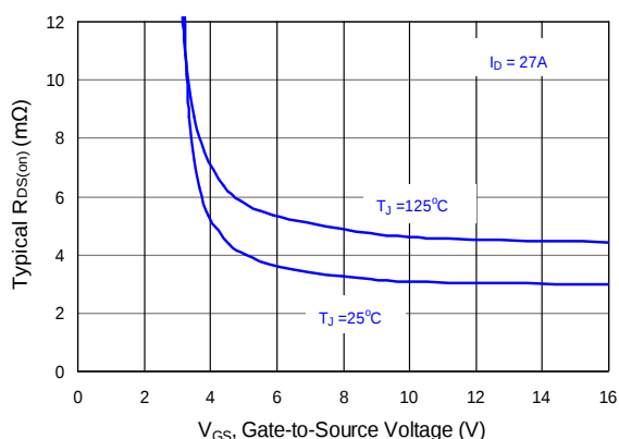
Figure 10: Q1 & Q3 Typical On-Resistance
