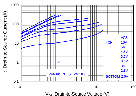
Figure 8: Q2 & Q4 Typical Output Characteristics @150°C
