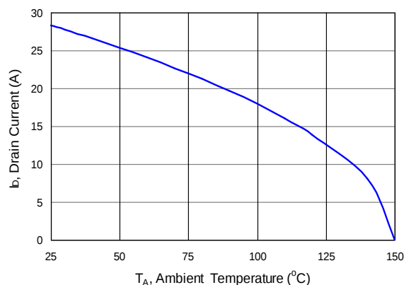
Figure 23: Q1 & Q3 Maximum Drain Current vs. Temperature
