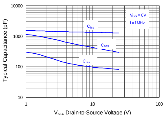
Figure 12: Q1 & Q3 Typical Capacitance vs. Drain-Source Voltage
