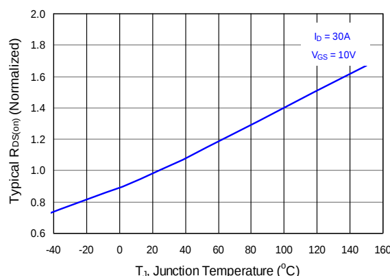
Figure 14: Q2 & Q4 On-Resistance vs. Temperature
