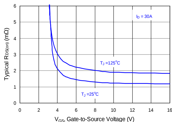
Figure 13: Q2 & Q4 Typical On-Resistance
