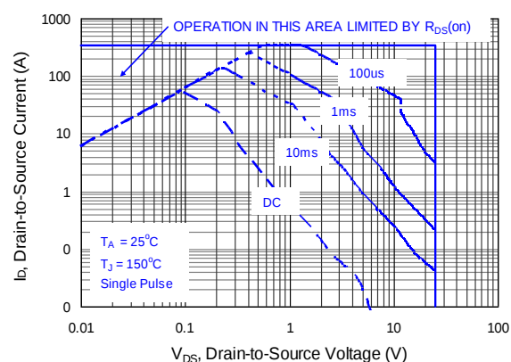
Figure 27: Q2 & Q4 Maximum Safe Operating Area
