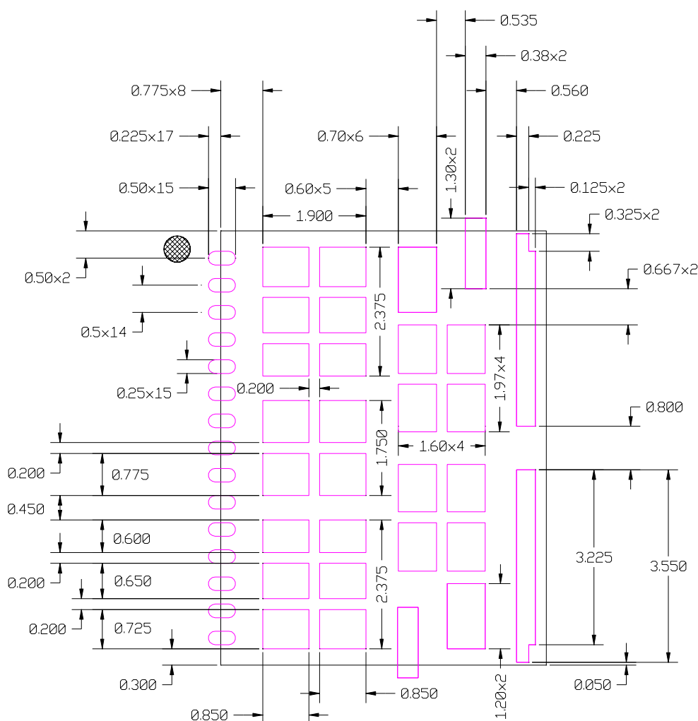
Figure 30: Stencil Design
