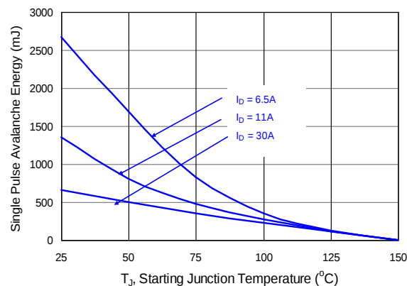
Figure 25: Q2 & Q4 Single Pulse Avalanche Energy
