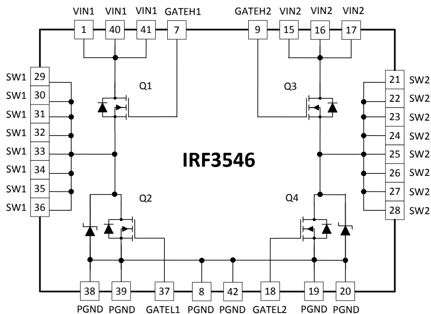
Figure 2: Block Diagram
