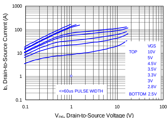
Figure 5: Q1 & Q3 Typical Output Characteristics @150°C
