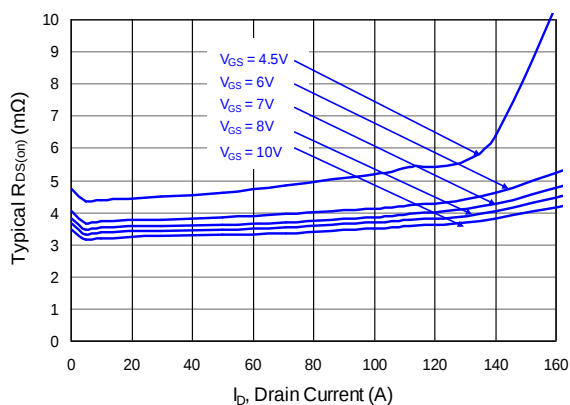
Figure 16: Q1 & Q3 Typical On-Resistance
