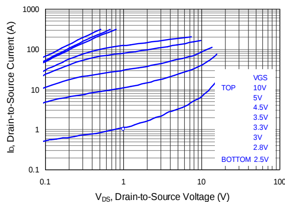
Figure 7: Q2 & Q4 Typical Output Characteristics
