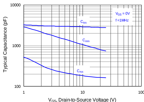
Figure 15: Q2 & Q4 Typical Capacitance vs. Drain-Source Voltage
