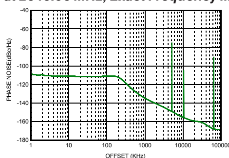
Figure 18. Fractional Spurious Performance at 2646.96 MHz, Exact Frequency Mode ON [11]
