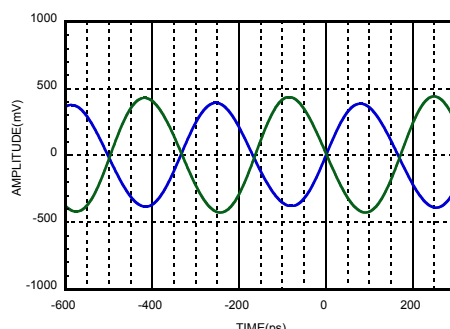
Figure 28. Phase Adjust at 180 degree [20]
