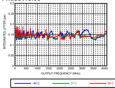
Figure 10. Single Sideband Integrated Phase Noise [7]
