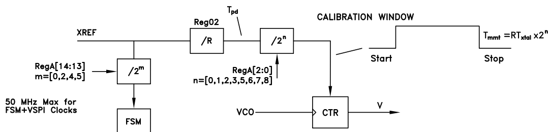
Figure 41. VCO Calibration
