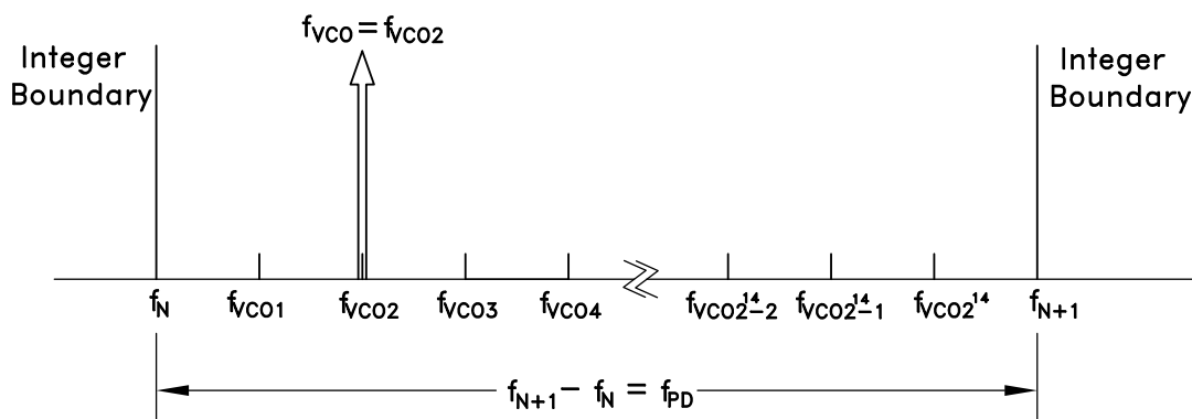
Figure 45. Exact Frequency Tuning
