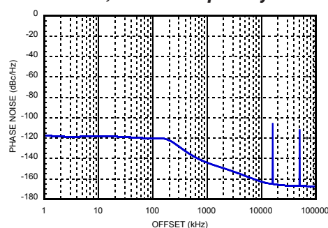
Figure 16. Fractional Spurious Performance at 904 MHz, Exact Frequency Mode ON [10]
