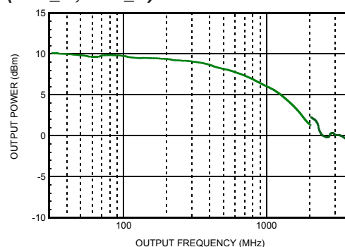
Figure 12. Single-Ended Output Power (LO1_N, LO2_P) [9]
