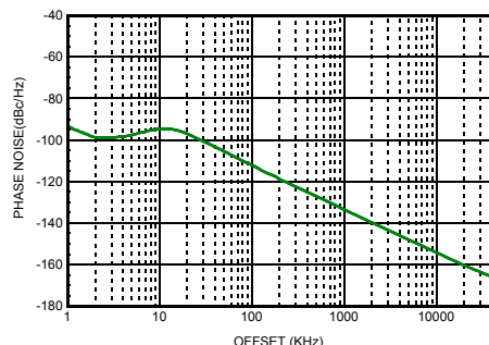
Figure 37. HMC835LP6GE with External VCO HMC384LP4E at 2213MHz [25]
