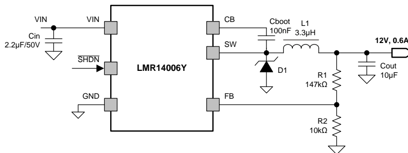
Figure 10. Application Circuit, 12 V Output
