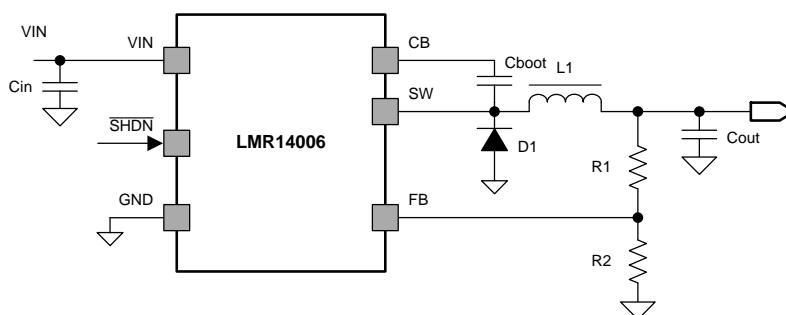
Figure 1. Typical Application Schematic
