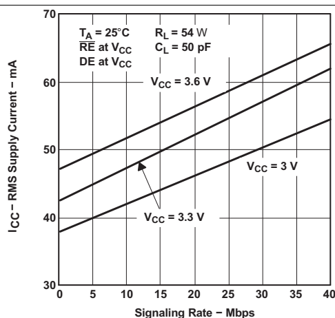
Figure 1. HVD10 RMS Supply Current vs Signaling Rate
