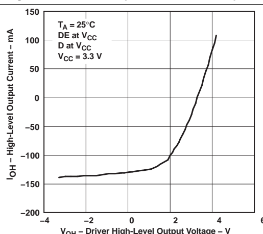
Figure 6. High-Level Output Current vs Driver High-Level Output Voltage
