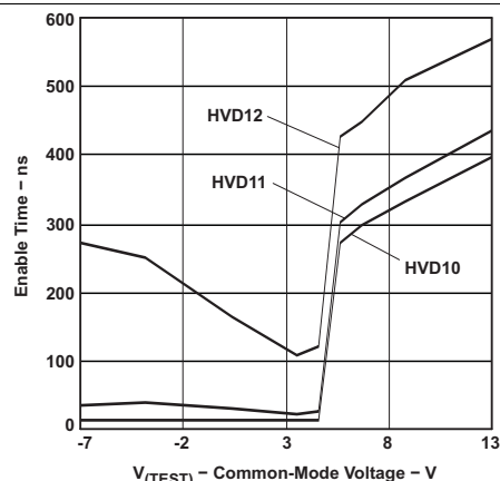
Figure 10. Enable Time vs Common-Mode Voltage
