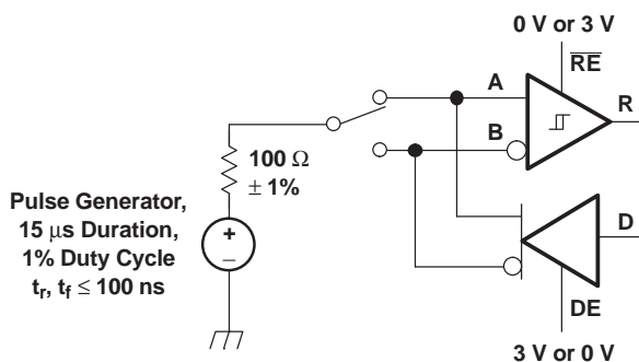
Figure 22. Test Circuit, Transient Over Voltage Test
