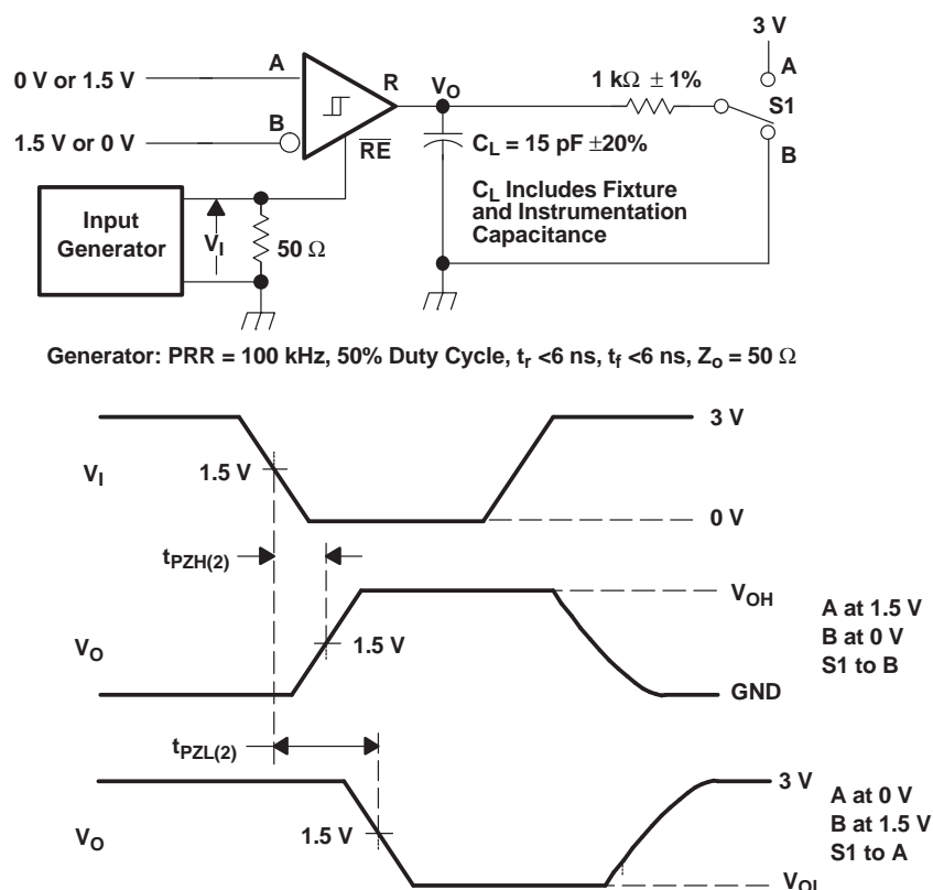
Figure 21. Receiver Enable Time From Standby (Driver Disabled)
