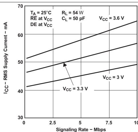
Figure 2. HVD11 RMS Supply Current vs Signaling Rate
