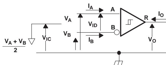
Figure 18. Receiver Voltage and Current Definitions
