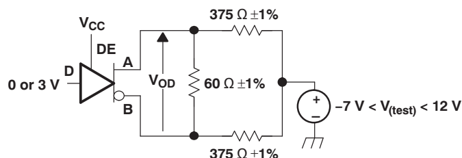
Figure 12. Driver V_{OD} With Common-Mode Loading Test Circuit
