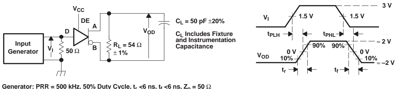
Figure 14. Driver Switching Test Circuit and Voltage Waveforms
