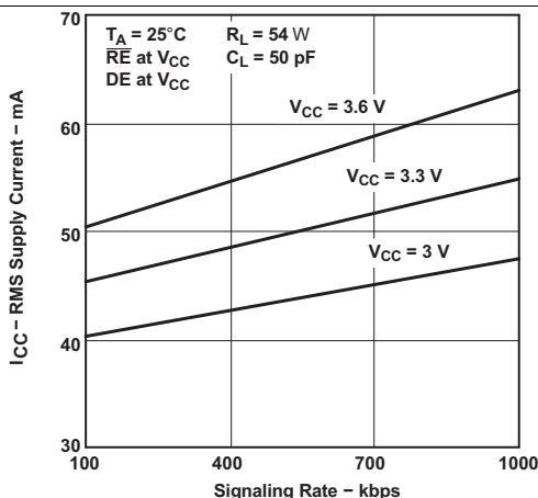
Figure 3. HVD12 RMS Supply Current vs Signaling Rate
