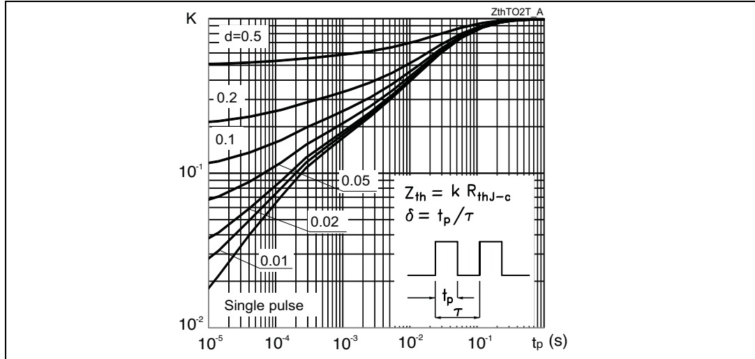
Figure 26. Thermal impedance for IGBT
