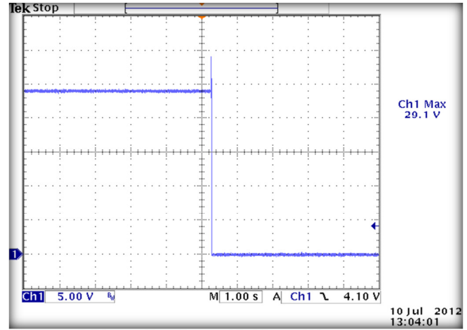
24V OUT, FULL LOAD, 264VAC, 50Hz
