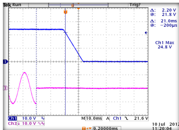
24V OUT, FULL LOAD, 120VAC, 60Hz
