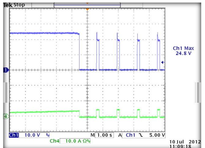
24V OUT, 264VAC
