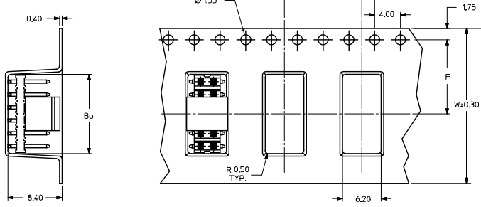
EMBOSSED CARRIER TAPE TYPE "B"
