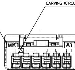
CARVING (CIRCUIT NO.1)
