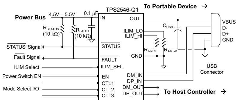
Figure 40. Typical Application Schematic USB Port Charging
