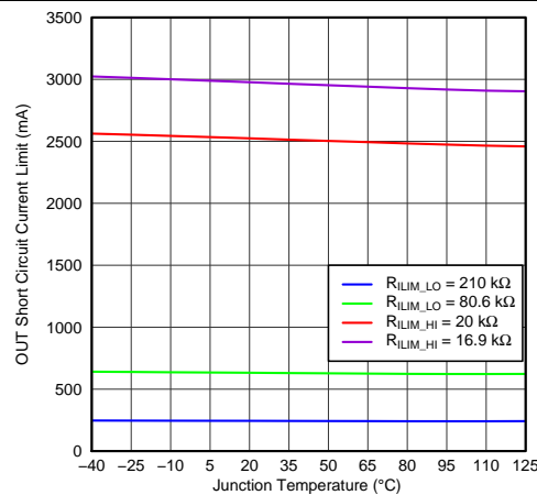
Figure 4. OUT Short-Circuit Current Limit vs Temperature
