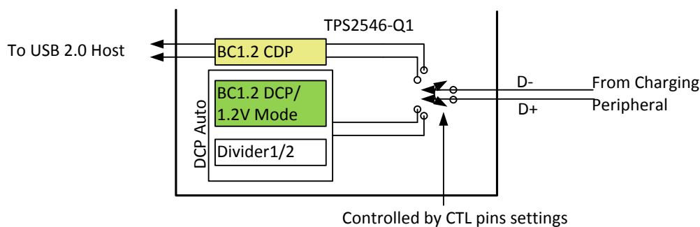
Figure 37. DCP Auto Mode
