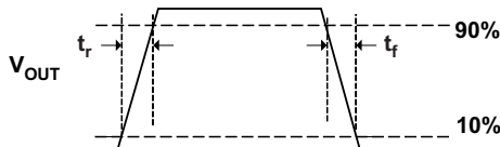
Figure 24. Power-ON and OFF Timing
