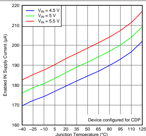
Figure 7. Enabled in Supply Current - CDP vs Temperature
