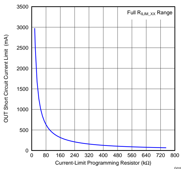
Figure 41. Typical Current Limit Setting vs Programming Resistor
