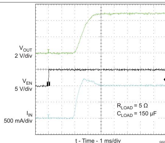
Figure 18. Turnon Response
