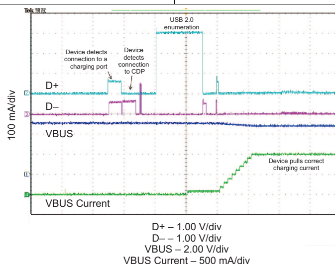
Figure 44. High-Current Limit
