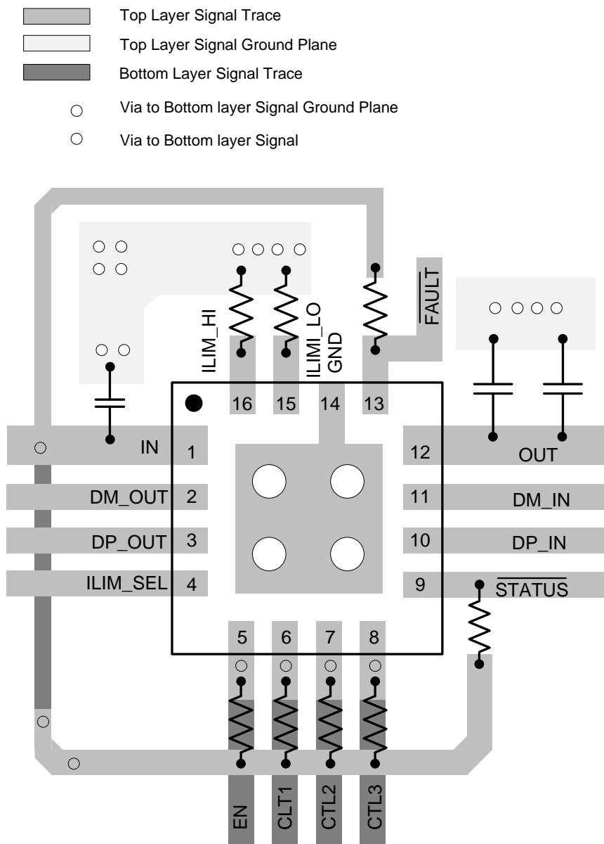
Figure 47. Layout Recommendation
