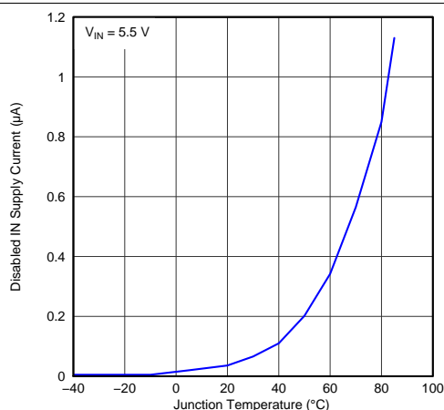
Figure 5. Disabled in Supply Current vs Temperature
