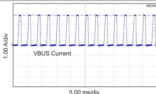
Figure 44. High-Current Limit
