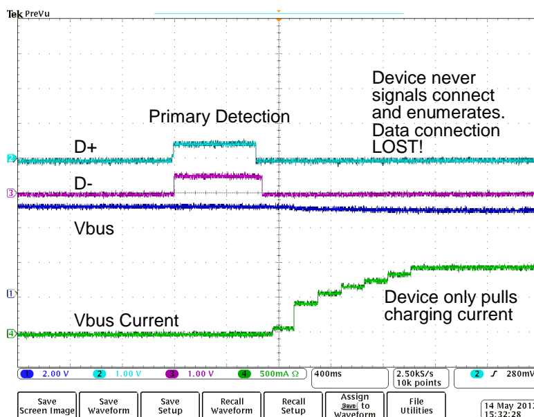
Figure 39. CDP/SDP Auto
