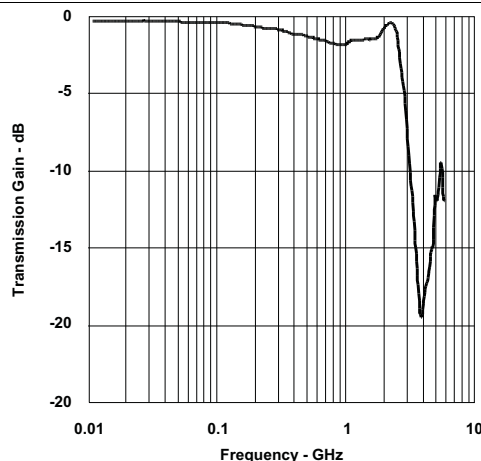
Figure 10. Data Transmission Characteristics vs Frequency
