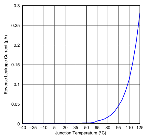
Figure 2. Reverse Leakage Current vs Temperature
