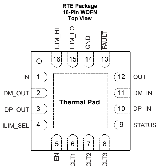
Pin Functions
