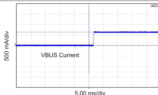
Figure 45. Low-Current Limit
