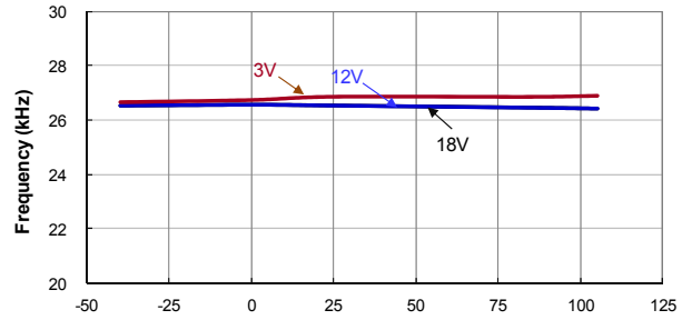
PWM Oscillator Frequency vs. Temperature
