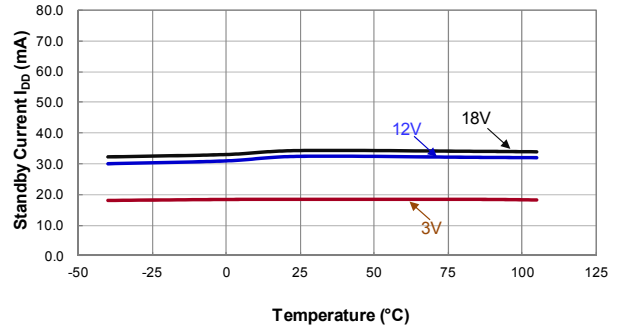
Standby Supply Current vs. Temperature
