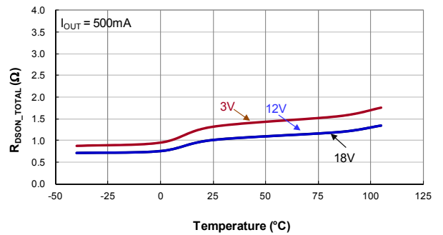
High+Low Side ON Resistance R_{DSON\_TOTAL} vs. Temperature
