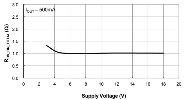
High+Low Side Resistance R_{DSON\_TOTAL} vs. Voltage
