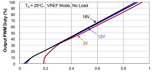
Output PWM Duty vs V_{REF}/V_{DD} Ratio
