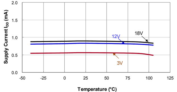
Supply Current vs. Temperature
