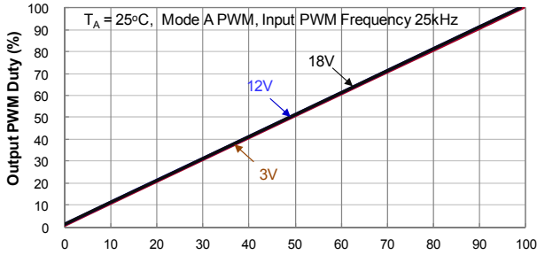
Output PWM Duty vs Input PWM Duty
