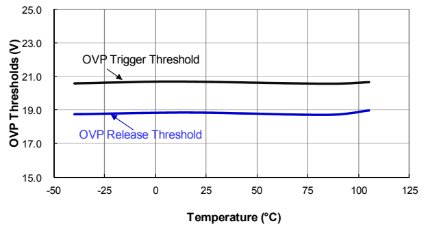
OVP Trigger and Release Thresholds vs Temperature
