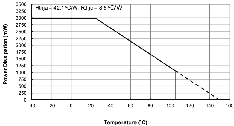
SO-8EP Thermal Derating Curve
