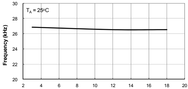
PWM Oscillator Frequency vs. Supply Voltage
