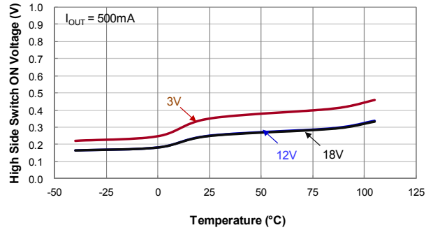
HighSide Switch On Voltage ( V_{DD}-V_{OL} ) vs. Temperature
