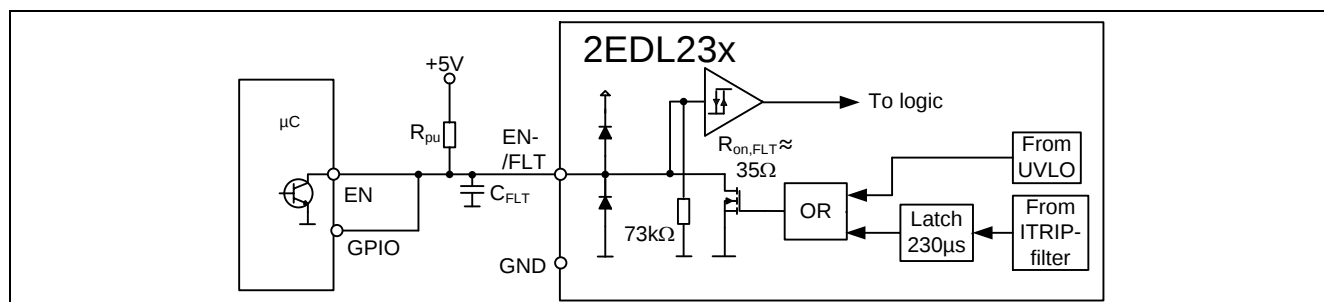
Figure 6 EN-/FLT pin structures and interface to microcontroller (μC)
