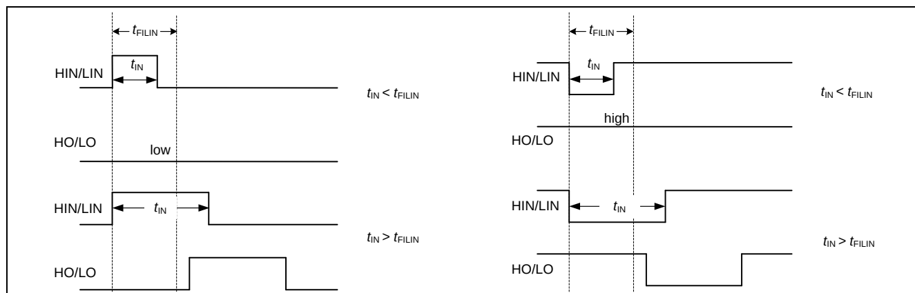
Figure 7 Timing of short pulse suppression
