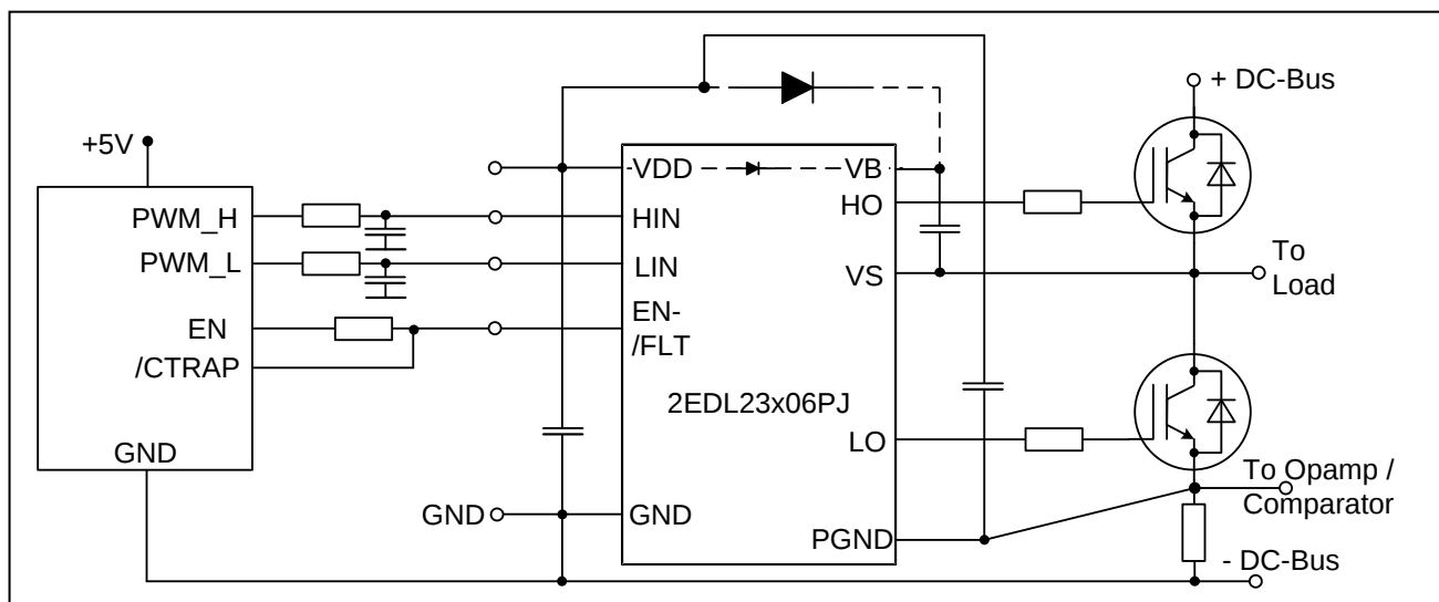
Figure 1 Typical Application
