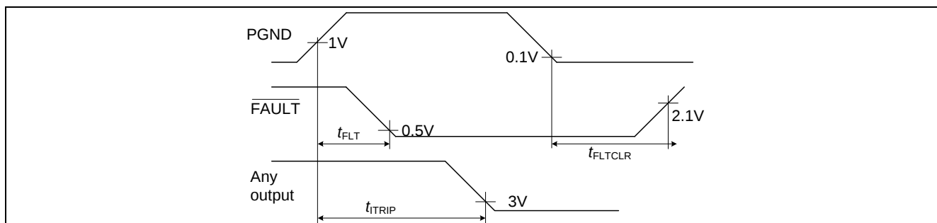
Figure 13 ITRIP-Timing
