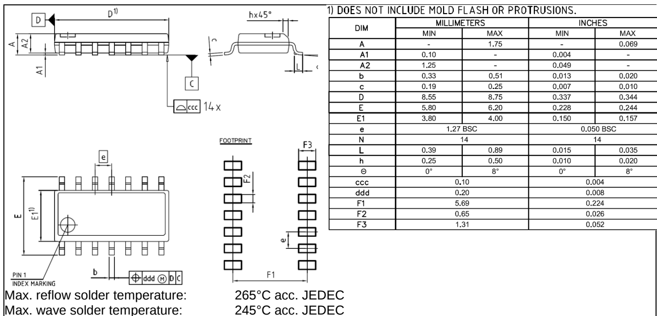
Figure 15 Package drawing
