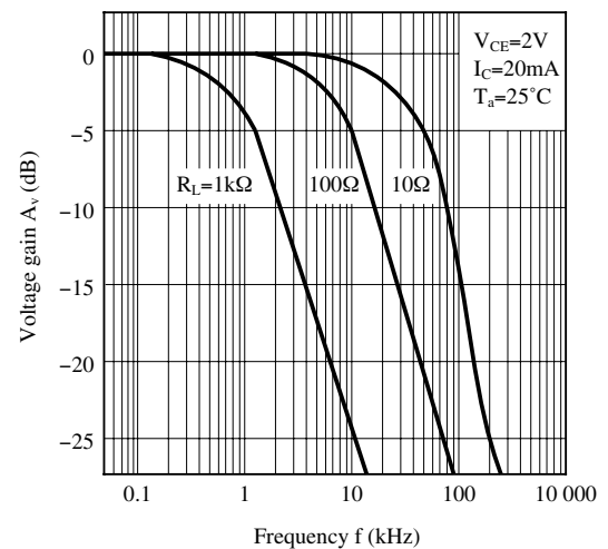
Fig.12 Frequency Response
