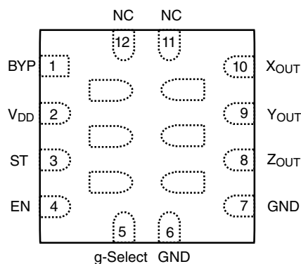
Figure 2. Pin locations
