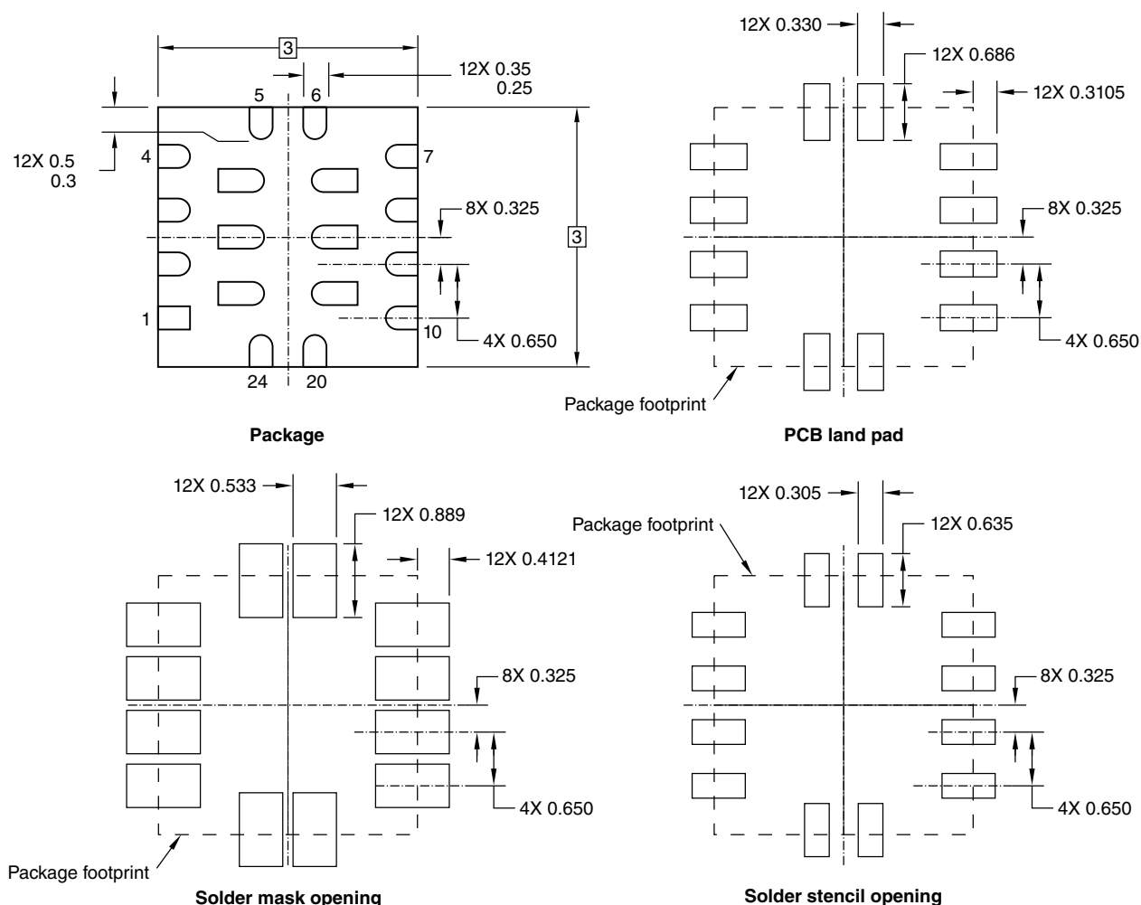
Figure 5. Footprint
