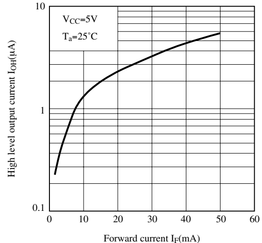
Fig.10 High Level Output Current vs. Forward Current
