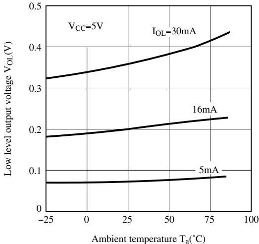
Fig.9 Low Level Output Voltage vs. Ambient Temperature
