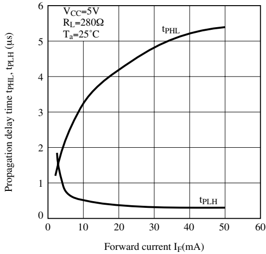
Fig.13 Propagation Delay Time vs. Forward Current
