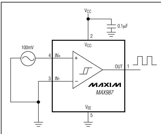
Figure 3. Zero-Crossing Detector
