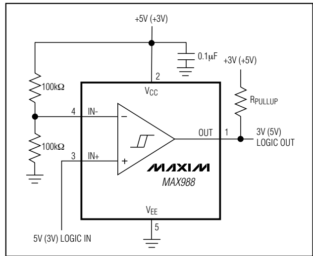
Figure 4. Logic-Level Translator
