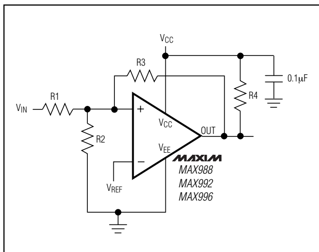
Figure 2. Additional Hysteresis (MAX988/MAX992/MAX996)
