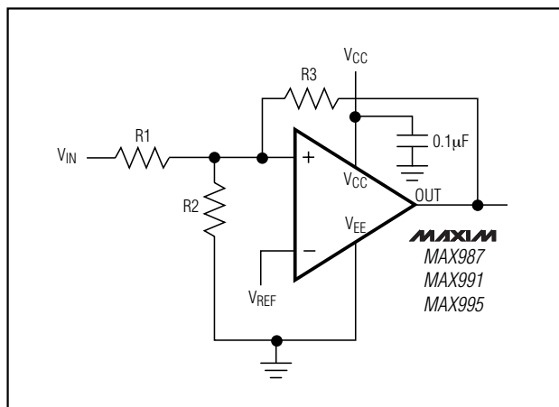
Figure 1. Additional Hysteresis (MAX987/MAX991/MAX995)
