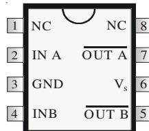
8 Lead PDIP (PI) 8 Pin SOIC (SI) IXDI404
