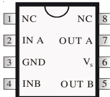
8 Lead PDIP (PI) 8 Pin SOIC (SI) IXDN404
