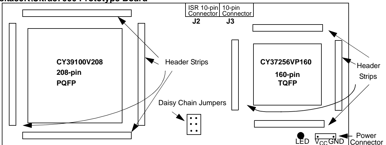
Figure 2. Delta39K\Ultra37000 Prototype Board
