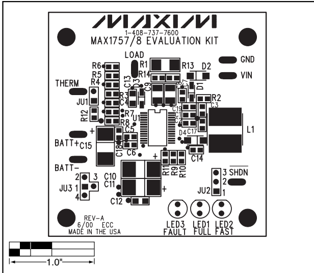
Figure 2. MAX1757/MAX1758 EV Kit Component Placement Guide—Component Side
