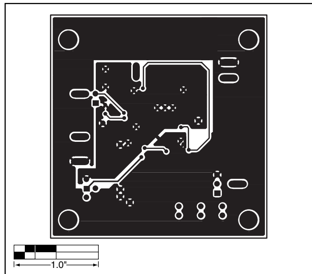
Figure 4. MAX1757/MAX1758 EV Kit PC Board Layout—Solder Side
