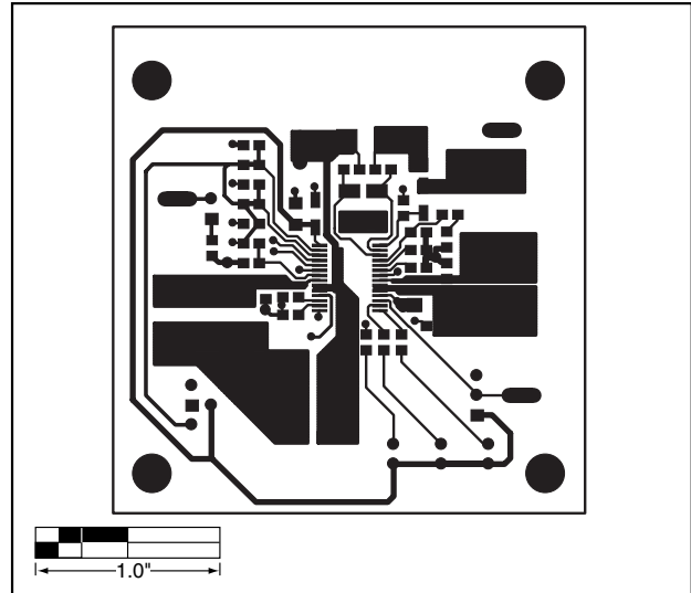
Figure 3. MAX1757/MAX1758 EV Kit PC Board Layout—Component Side
